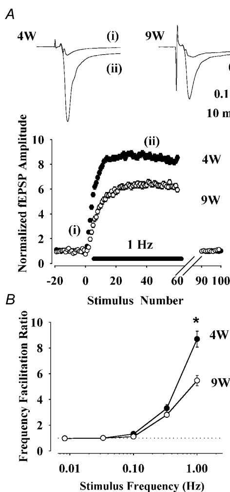
Figure 2. Developmental change in FFR
