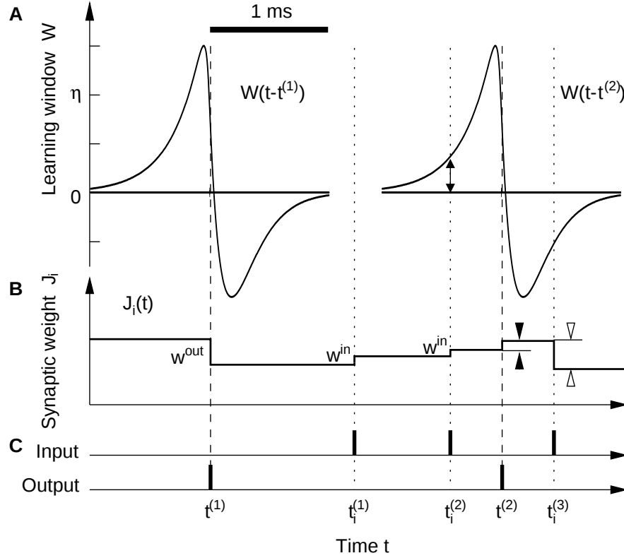
Figure 2: Spike-based learning. (A) Two plots of the learning window W in units of the learning parameter \eta as a function of the temporal difference between spike arrival at time t at synapse i (e.g., t = t_i^{(m)} , m = 1, 2, 3 ; dotted lines) and postsynaptic firing at times t^{(1)} and t^{(2)} (dashed lines). Scale bar = 1 ms. (B) Time course of the synaptic weight J_i(t) evoked through input spikes at synapse i and postsynaptic output spikes (vertical bars in C). The output spike at time t^{(1)} decreases J_i by an amount w^{out} . The input at t_i^{(1)} and t_i^{(2)} increase J_i by w^{in} each. There is no influence of the learning window W because these input spikes are too far away in time from t^{(1)} . The output spike at t^{(2)} , however, follows the input at t_i^{(2)} closely enough, so that, at t^{(2)} , J_i is changed by w^{out} < 0 plus W(t_i^{(2)} - t^{(2)}) > 0 (double-headed arrow), the sum of which is positive (filled arrowheads). Similarly, the input at t_i^{(3)} leads to a decrease w^{in} + W(t_i^{(3)} - t^{(2)}) < 0 (open arrowheads). The assumption of instantaneous and discontinuous weight changes can be relaxed to delayed and continuous ones that are triggered by spikes, provided weight changes are fast when compared with the time scale of learning [46]. If the integral \int_{-\infty}^{+\infty} W(s) ds is sufficiently negative, then one can drop w^{out} [49].
